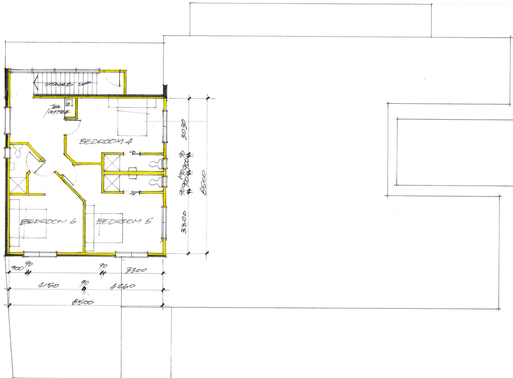
UPPER FLOOR PLAN 1:100
